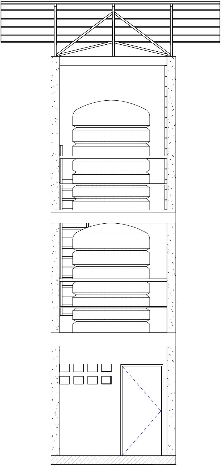
FACADE ARRIERE
